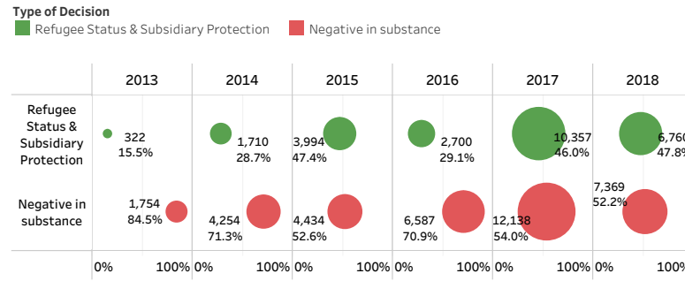
Recognition rate
